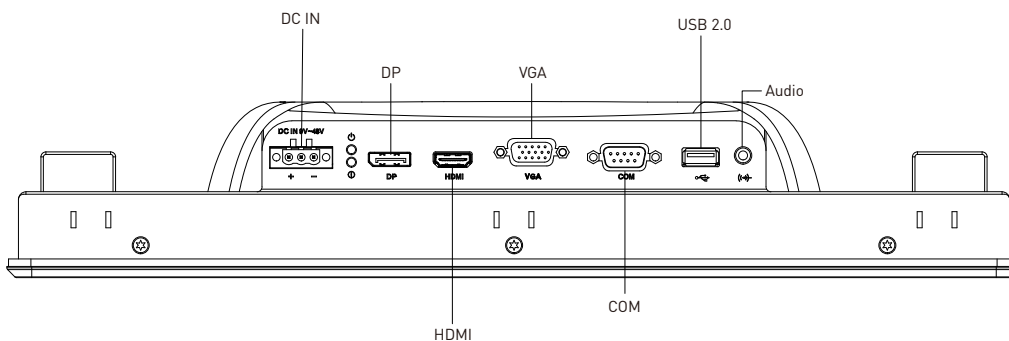
Rear I/O
